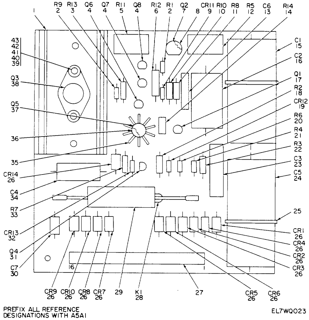
Figure 23. -25 +15 Volt Power Supply A5A1
