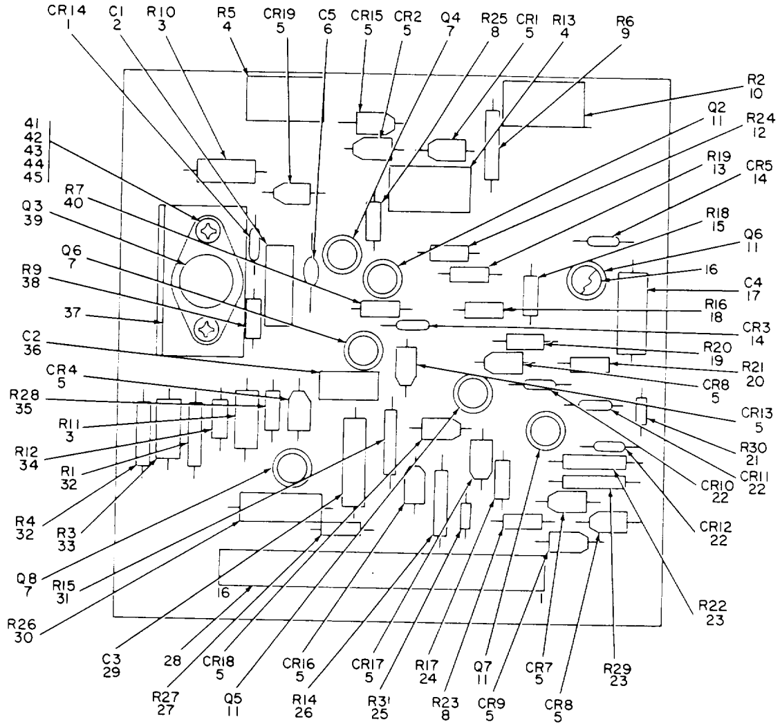
Figure 10. Series Passive Drive Assembly A4A3.
