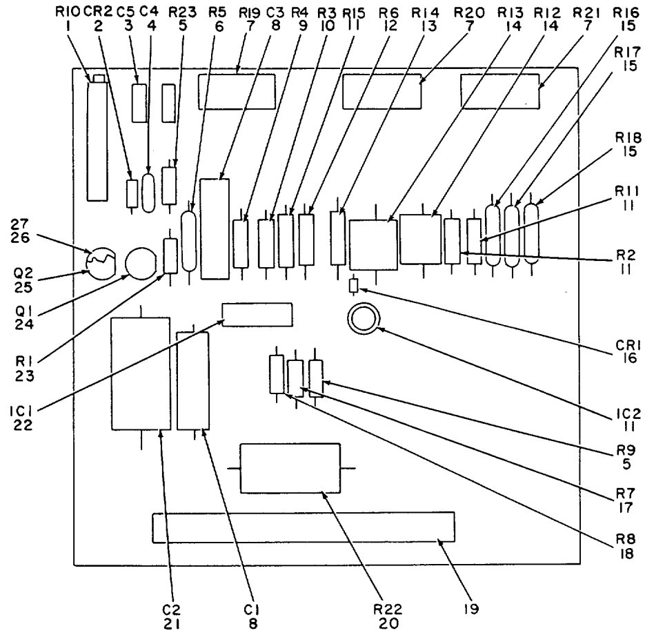
Figure 7. +10V Ref Supply A4A1.
