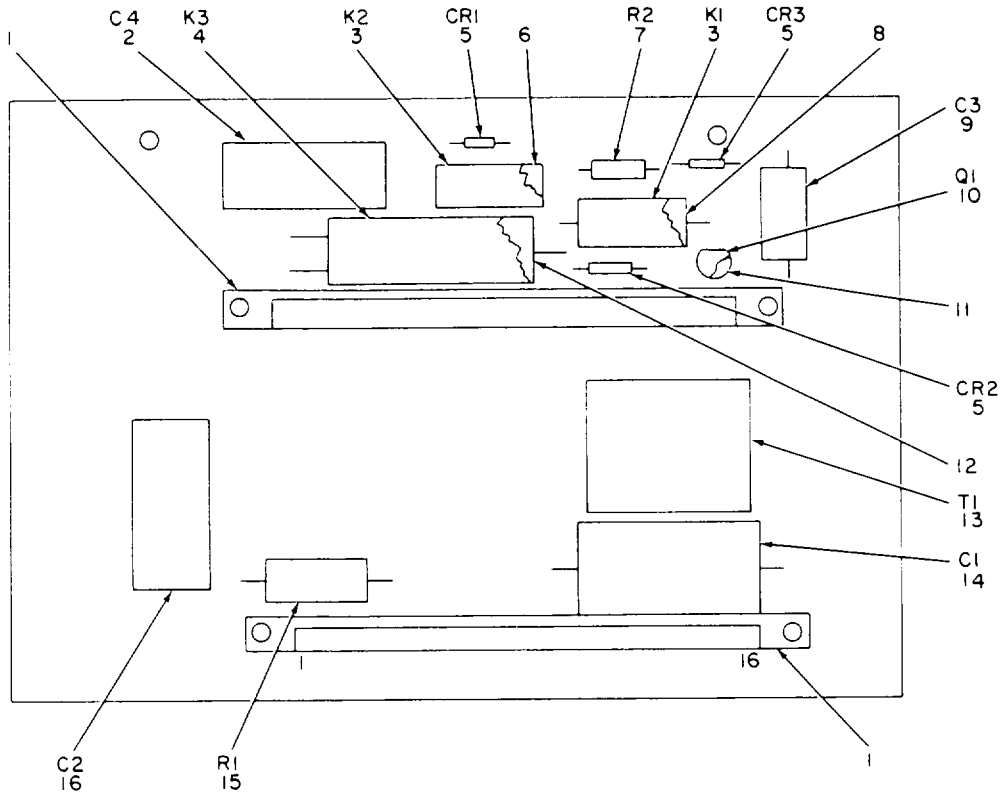
Figure 22. Rear Mother Board A5
