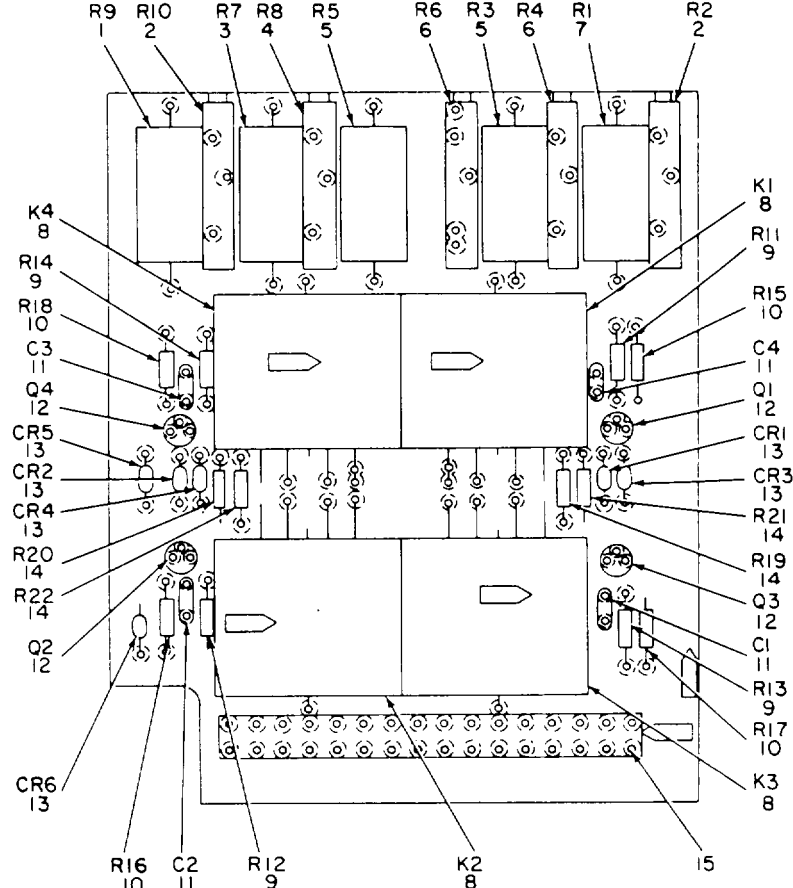
Figure 17. Ladder Driver 2 A4A11
