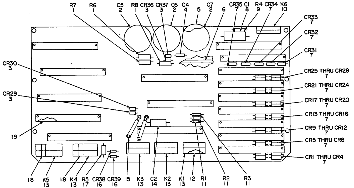
Figure 6. Main Mother Board A4.
