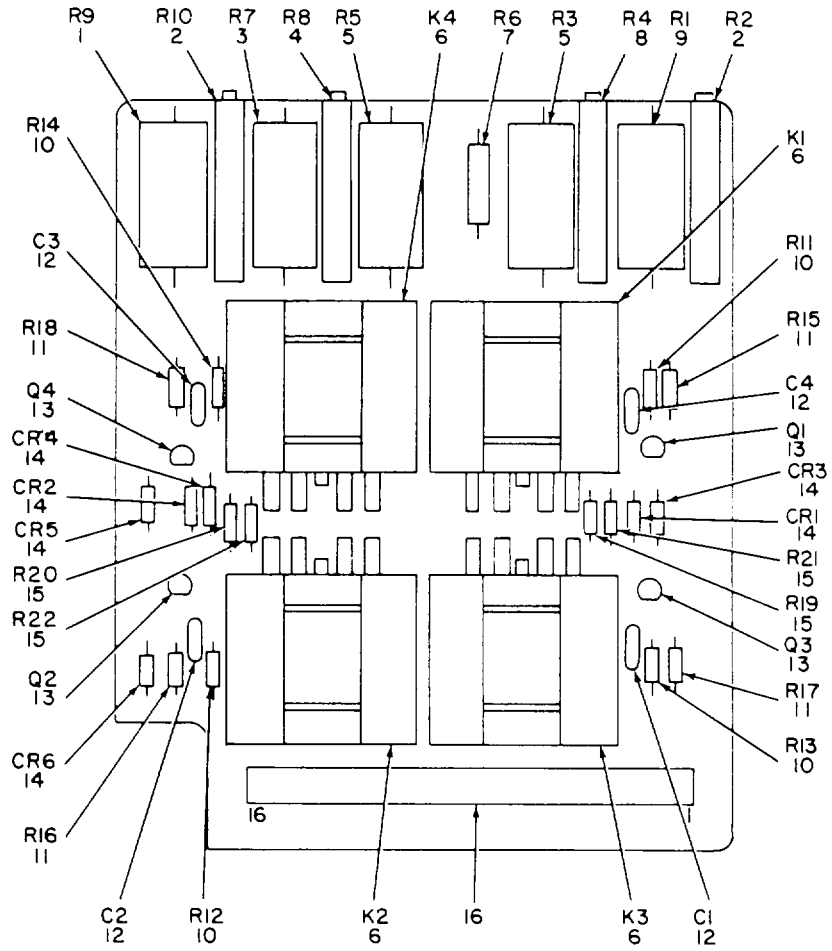
Figure 16. Ladder Driver 1 A4A10.
