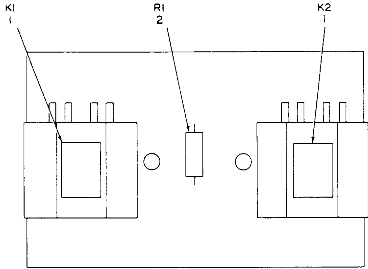
Figure 25. Relay Board Assembly A6
