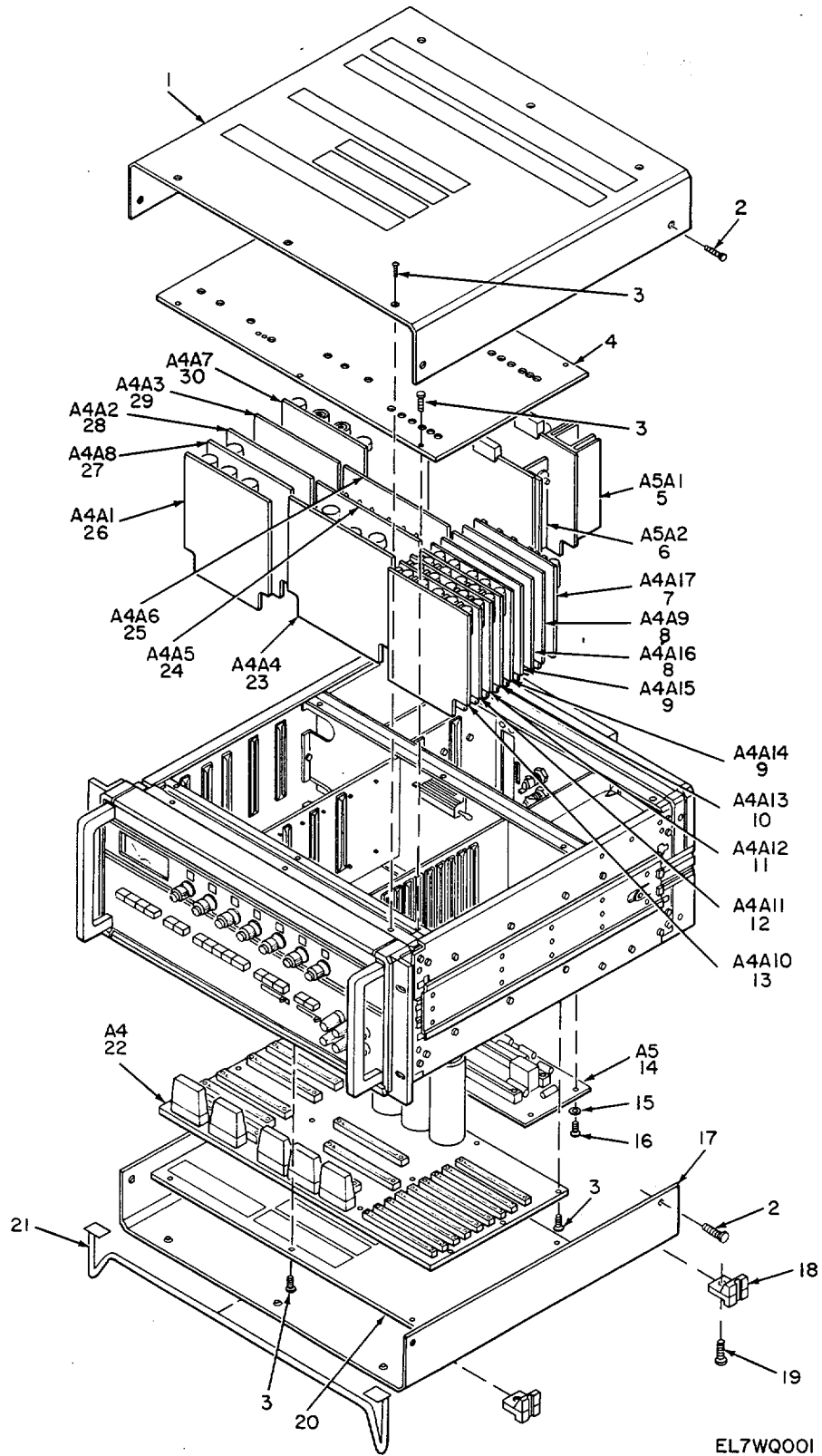
Figure 1. Calibrator, Direct Current 0-1805/USM (Sheet 1 of 4).
