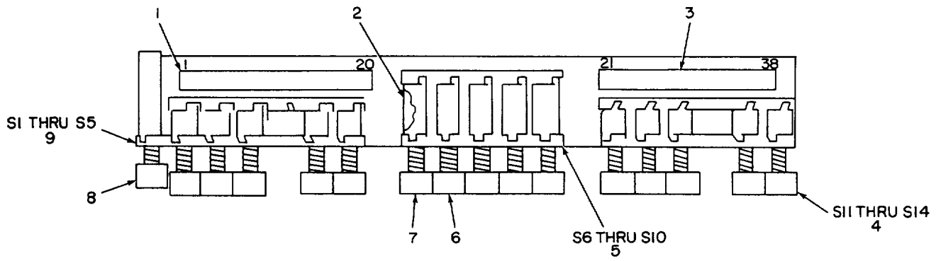
Figure 4. Switch Board Assembly A3A2.
