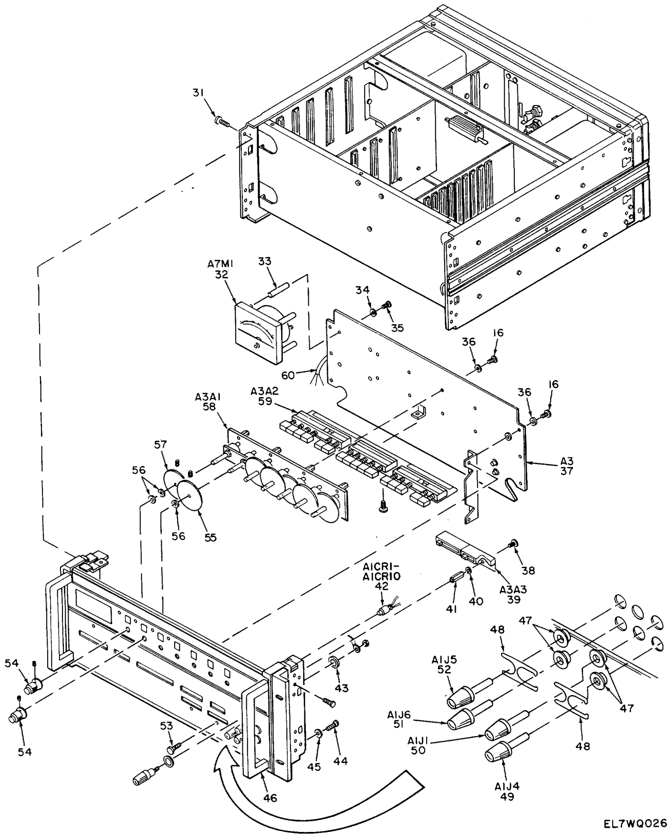
Figure 1. Calibrator, Direct Current 0-1805/USM (Sheet 2 of 4).
