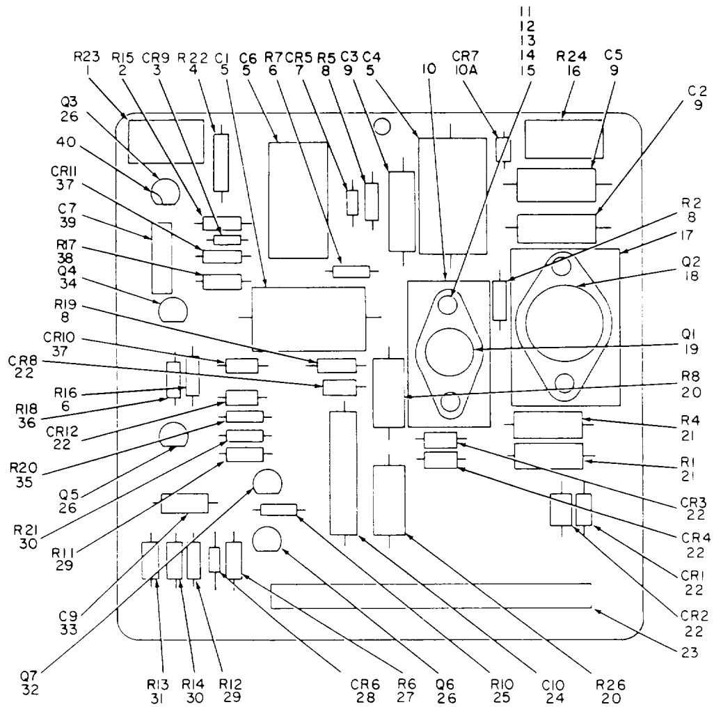
Figure 13. Current Limiter Assembly A4A7.
