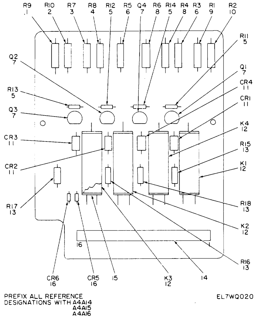
Figure 20. Ladder Driver 5 A4A14, 6 A4A15 and 7 A4A16
