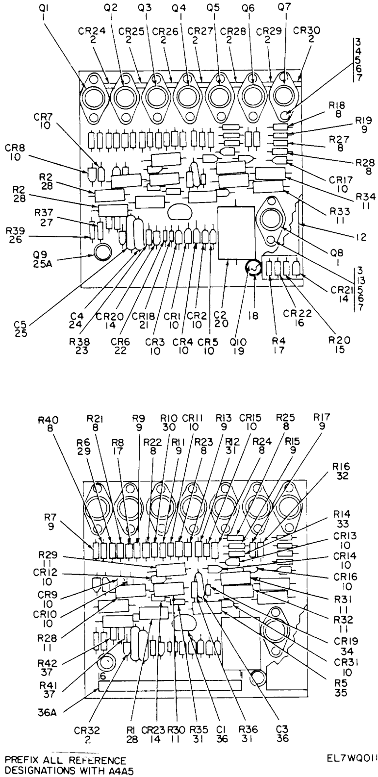
Figure 11. Series Passive Element A4A5.
