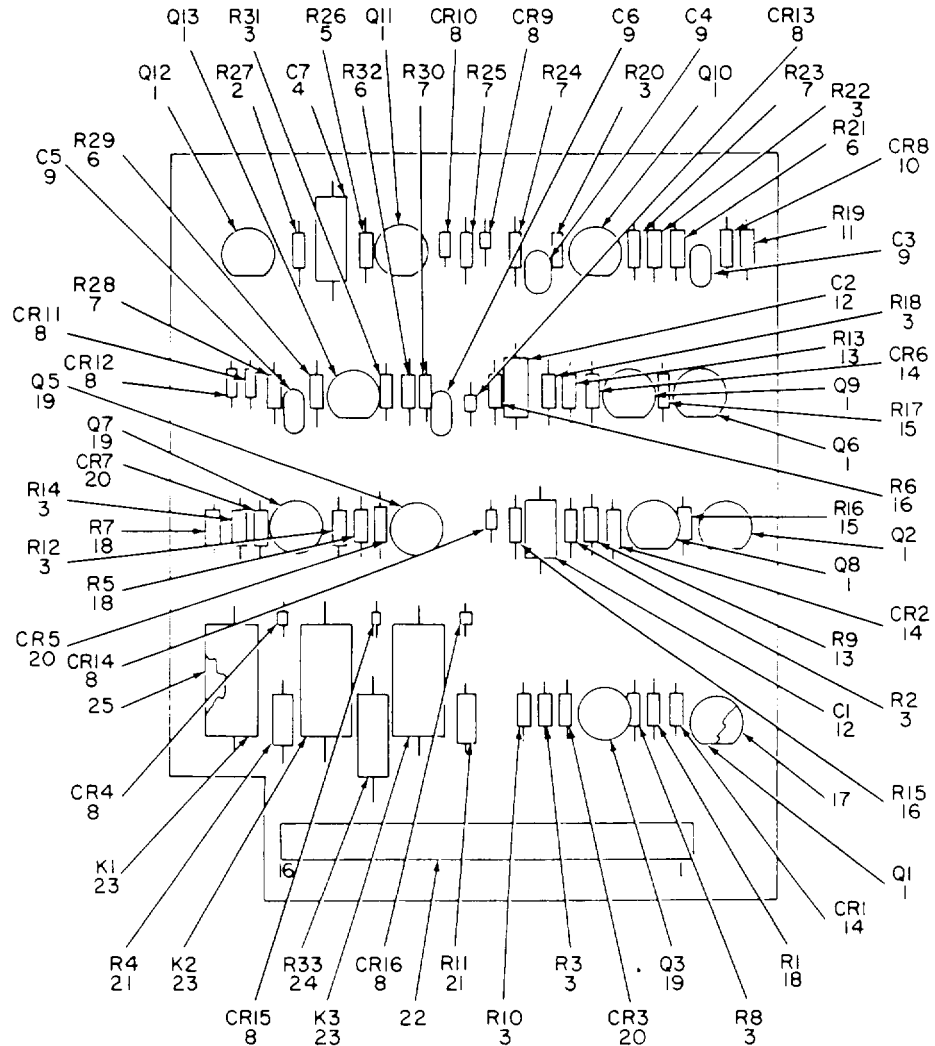
Figure 15. Relay Driver Assembly A4A9.
