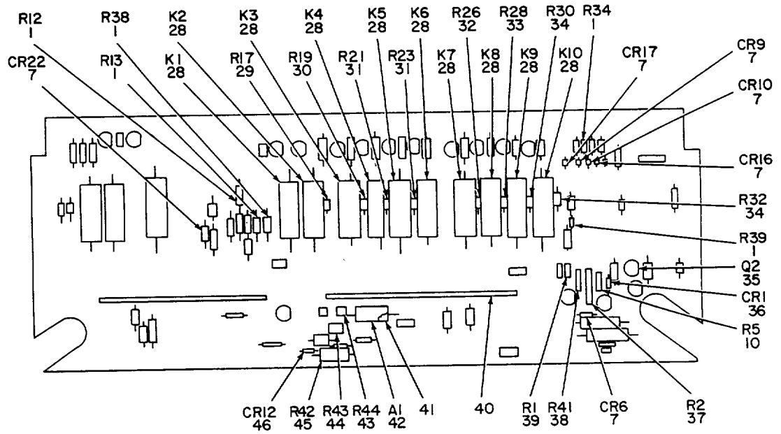
Figure 2. Front Mother Board Assembly.
