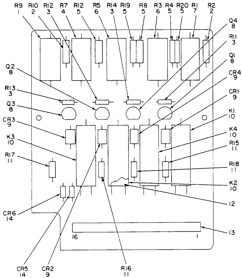
Figure 19. Ladder Driver 4 A4A13
