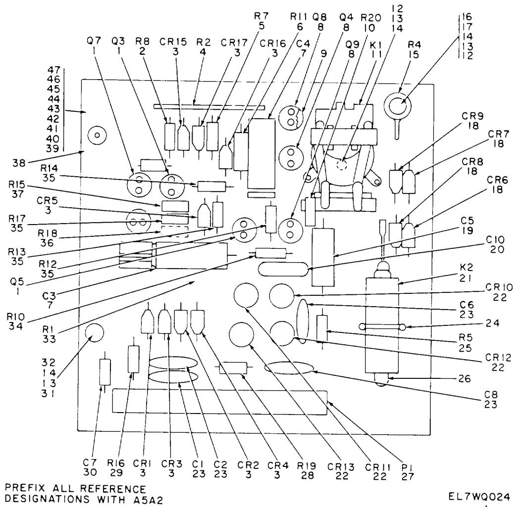
Figure 24. Preregulator Assembly A5A2
