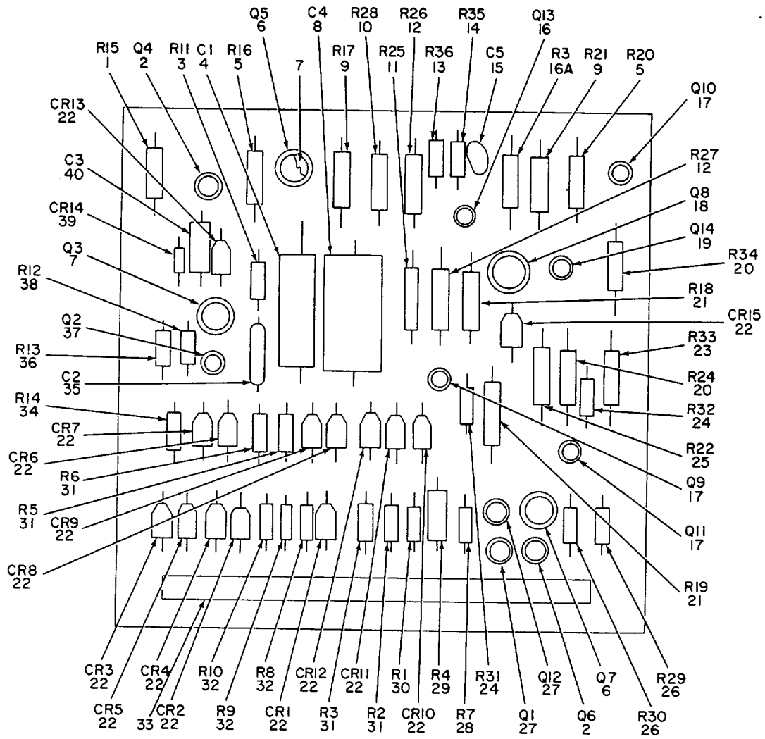
Figure 9. Differential Assembly A4A3.
