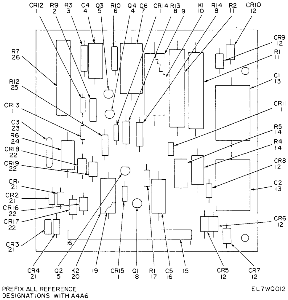
Figure 12. High Voltage Power Supply A4A6.
