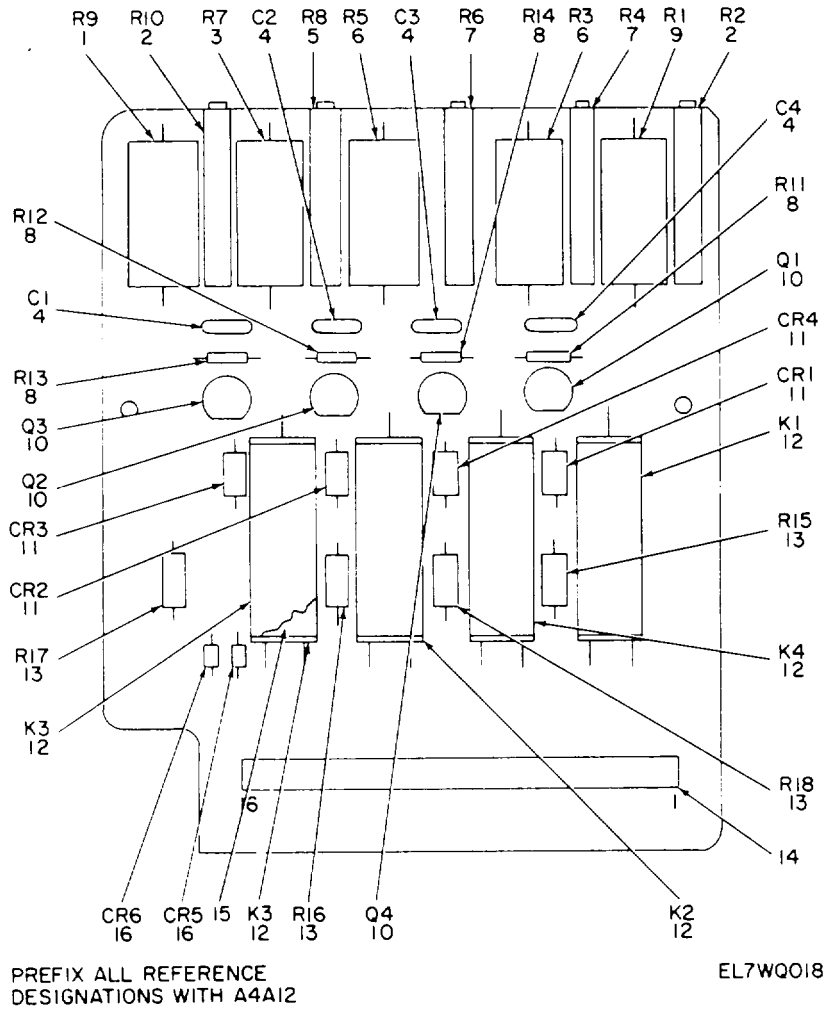
Figure 18. Ladder Driver 3 A4A12
