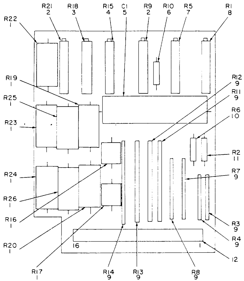
Figure 21. Range Shunt Assembly A4A17
