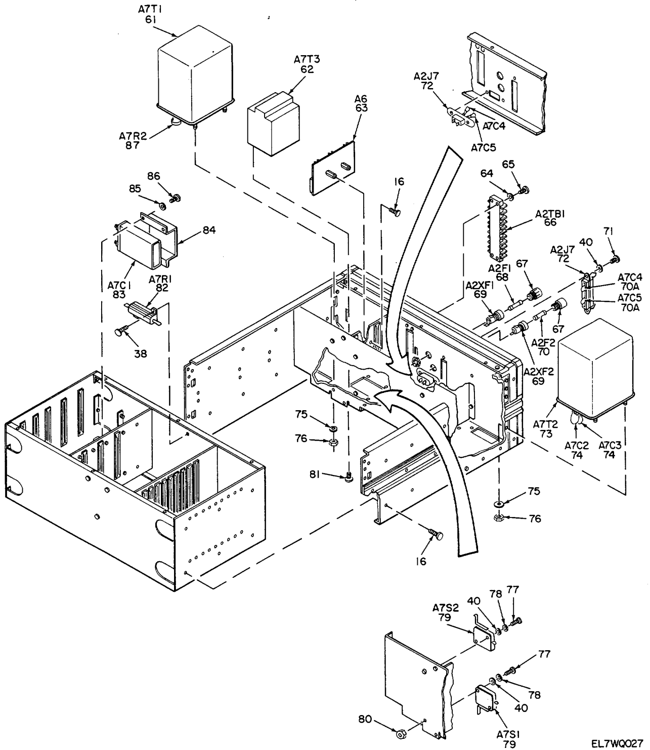
Figure 1. Calibrator, Direct Current 0-1805/USM (Sheet 3 of 4).
