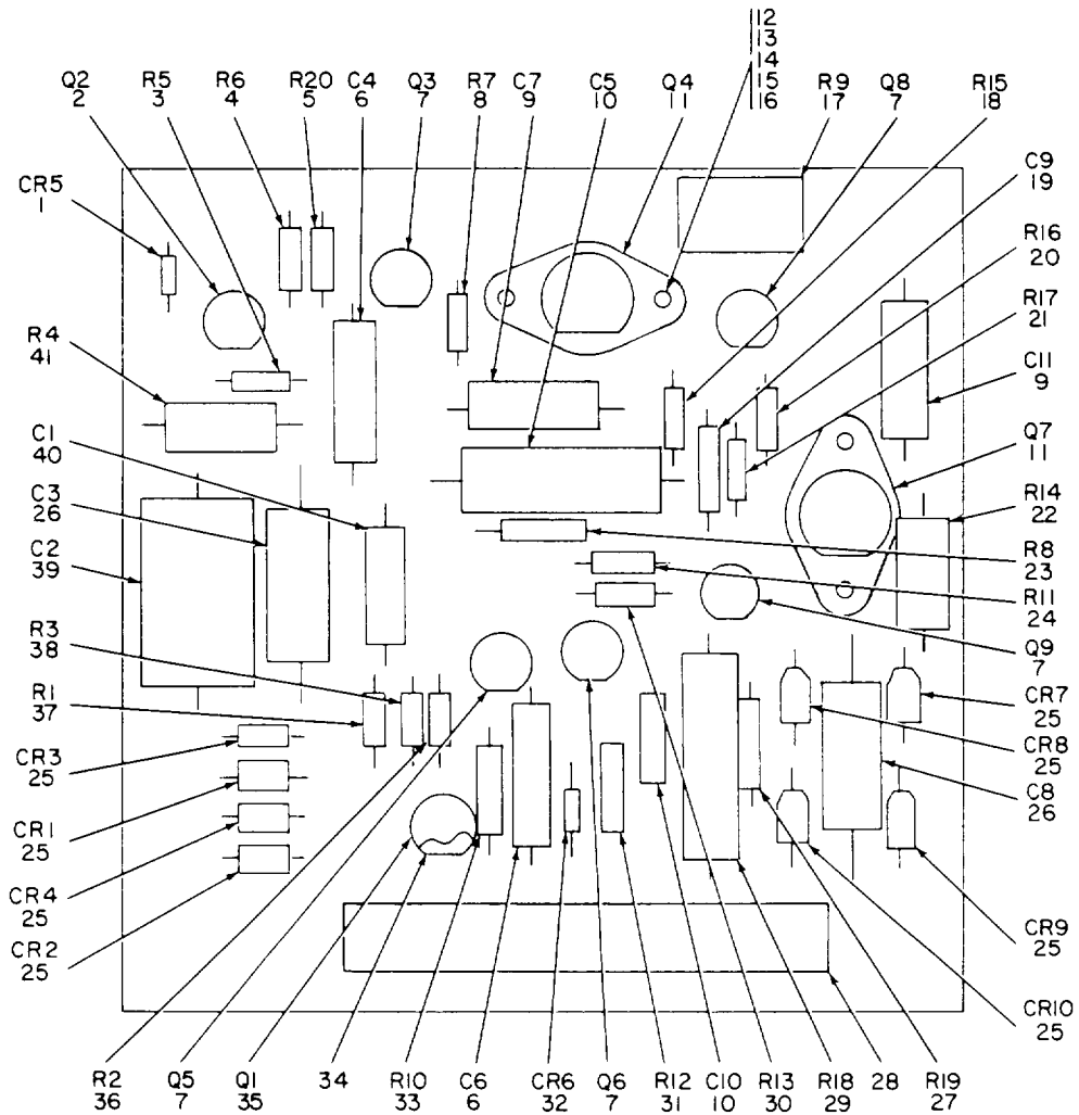
Figure 14. +25, -15 Power Supply A4A8.
